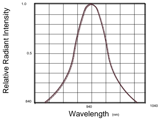
Fig.1 Spectral Distribution
