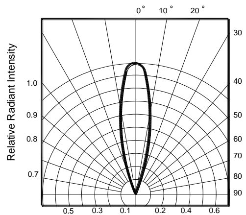
FIG.6 Radiant Diagram
