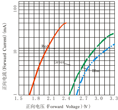
伏安特性 Volt-Ampere Characteristics T Ambient =25°C
