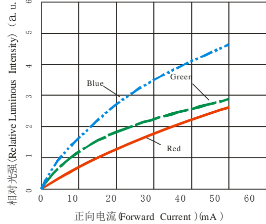
相对光强与正向电流特性 Relative Luminous Intensity VS Forward Current T Ambient =25°C
