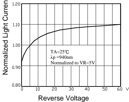
Normalized Light Current vs Reverse Voltage
